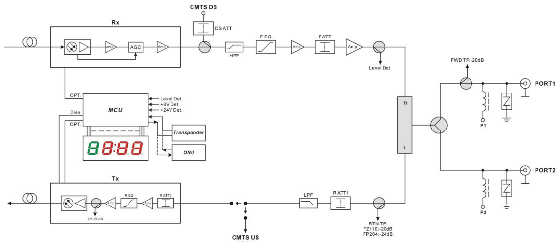
Dual Fiber Option
