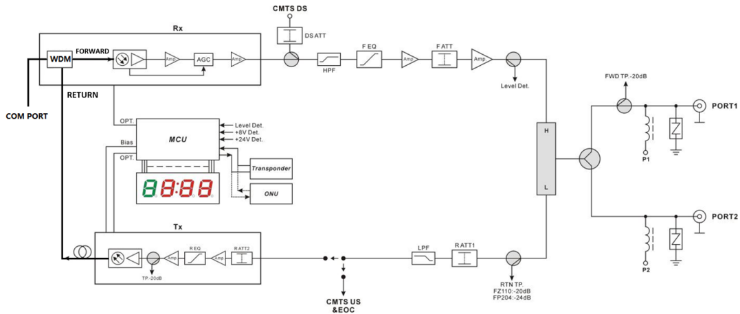
Single Fiber Option
